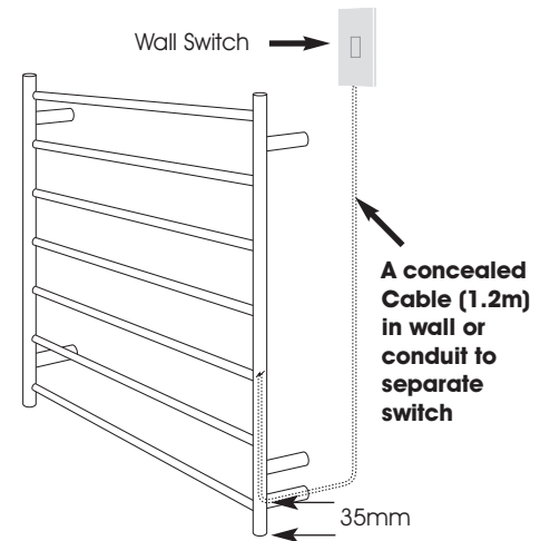
Hard Wired Concealed Cable
