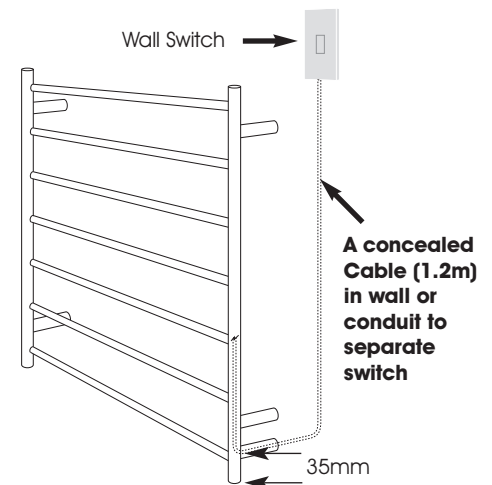
Hard Wired Concealed Cable
